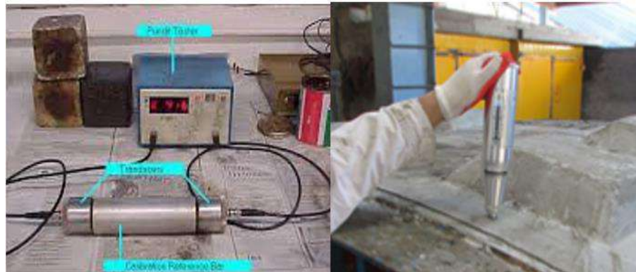
Figure 2: Ultrasonic Pulse Velocity Meter & Schmidt Hammer
